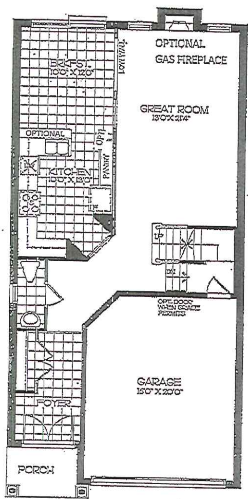
GROUND FLOOR 900 SF GFA 3000
