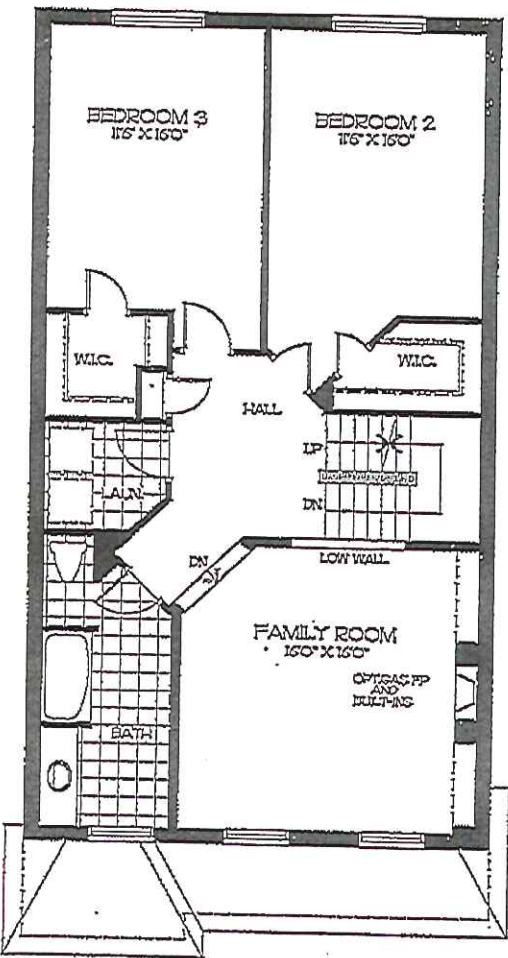
SECOND FLOOR 1200 SF
