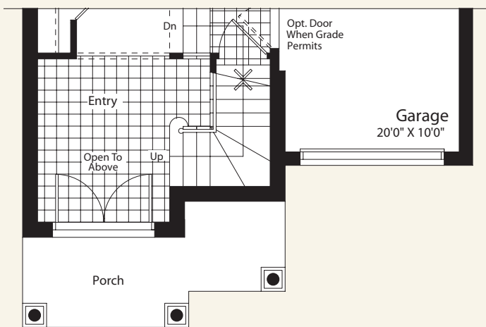
Ground Floor Elevation B
