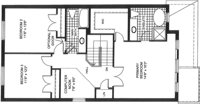
SECOND FLOOR ELEVATION 'B'
