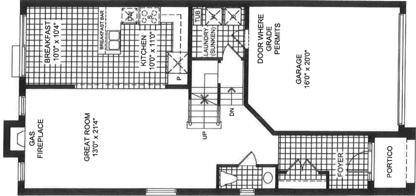
GROUND FLOOR ELEVATION 'B'
