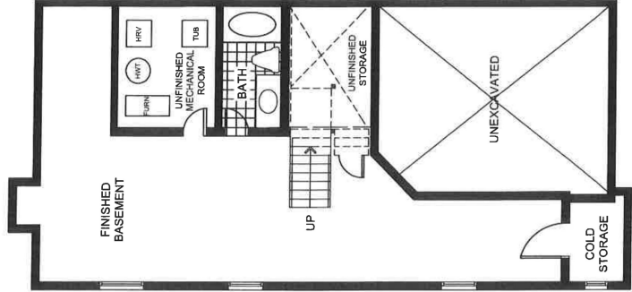
BASEMENT ELEVATION 'B'
