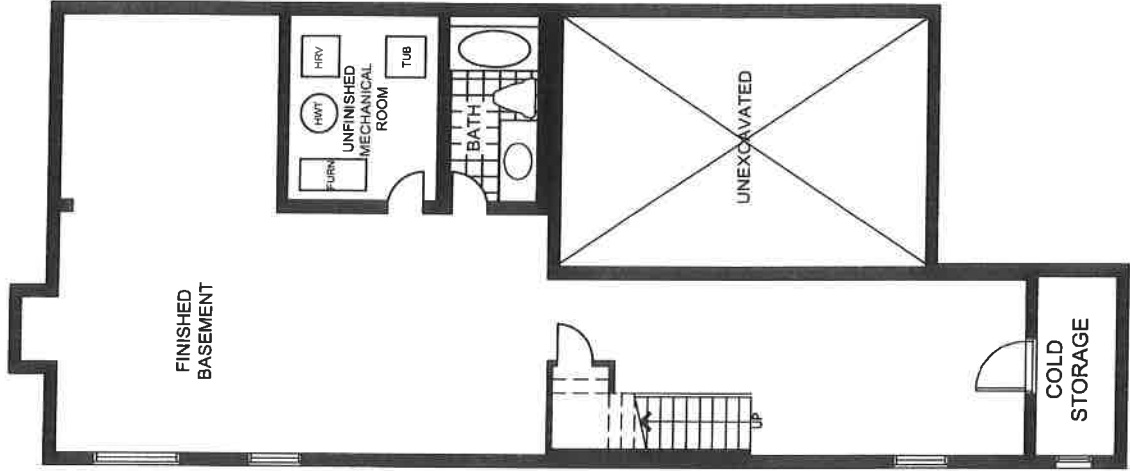
BASEMENT ELEVATION 'A'
