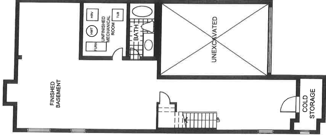
BASEMENT ELEVATION 'B'
