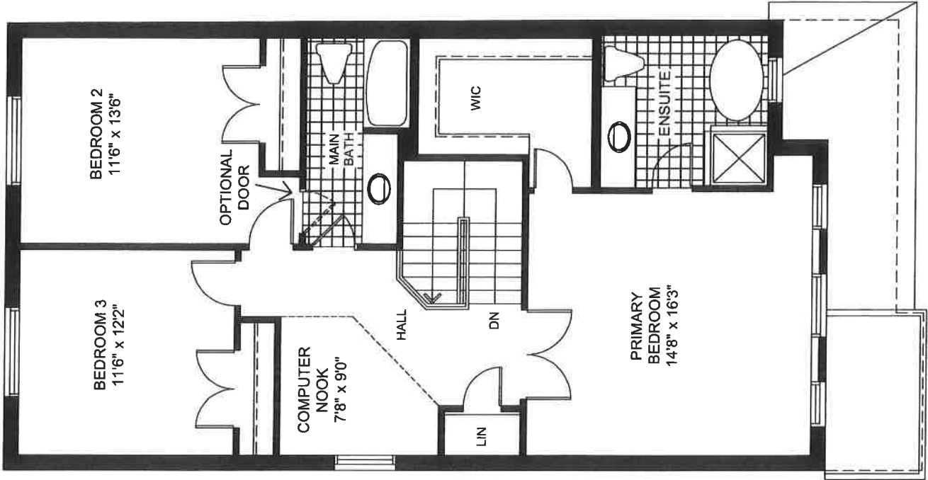
SECOND FLOOR ELEVATION 'B'
