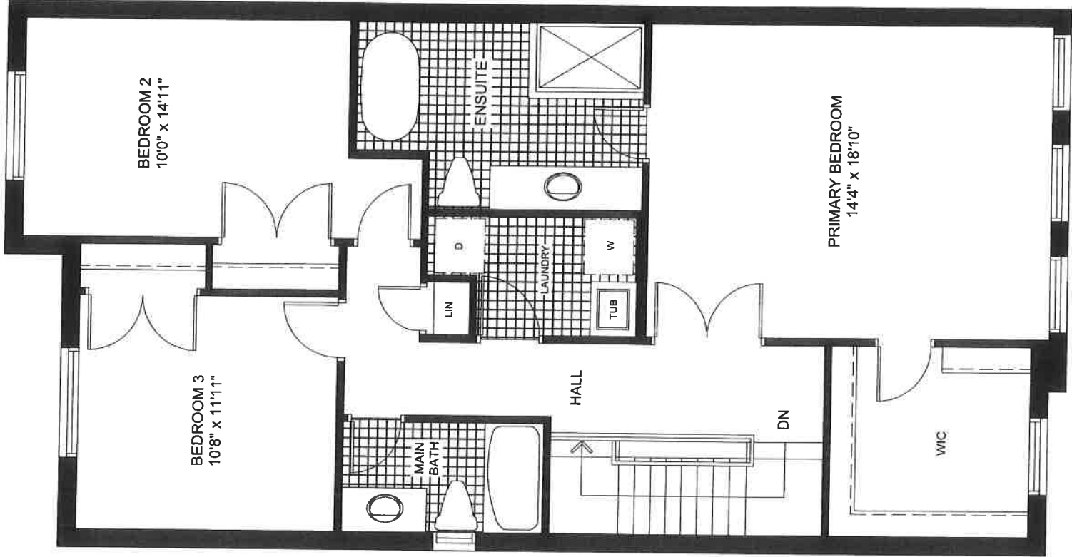
SECOND FLOOR ELEVATION 'B'
