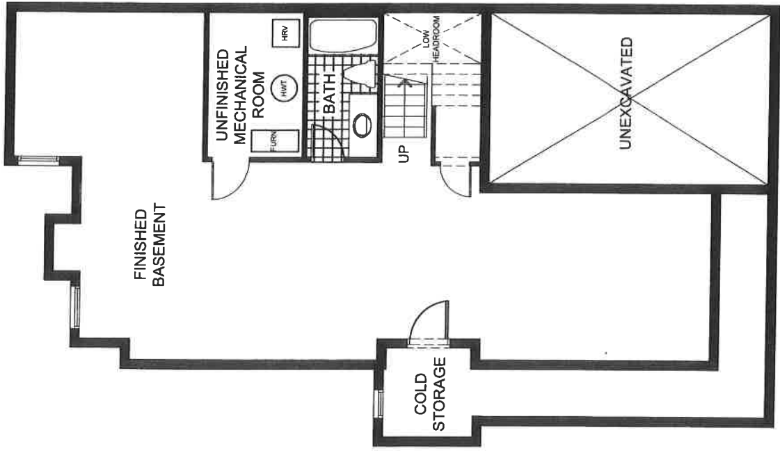
BASEMENT ELEVATION 'C'
