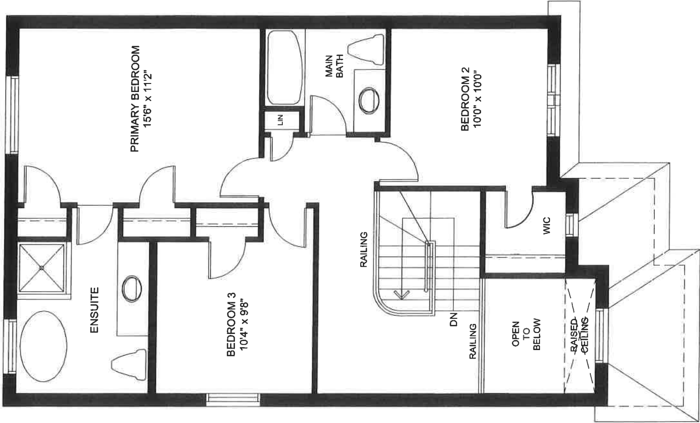
SECOND FLOOR ELEVATION 'B'
