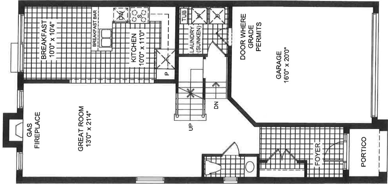
GROUND FLOOR ELEVATION 'B'
