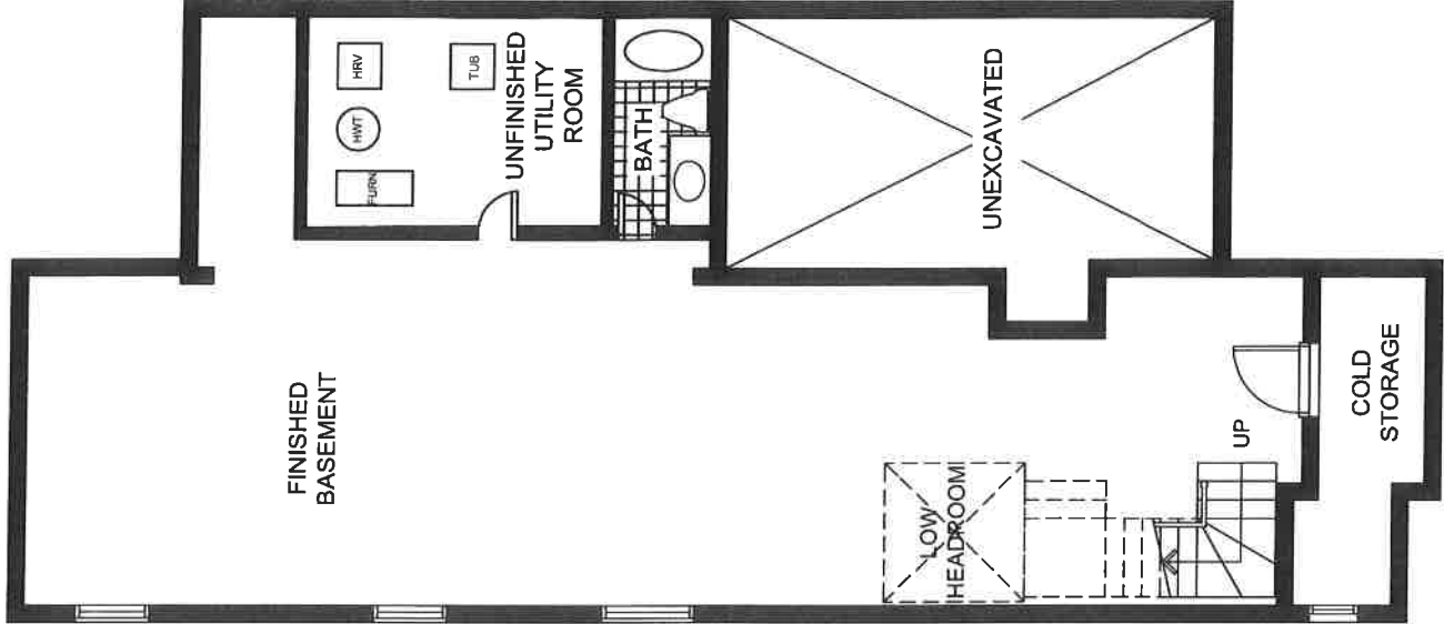
BASEMENT ELEVATION 'B'
