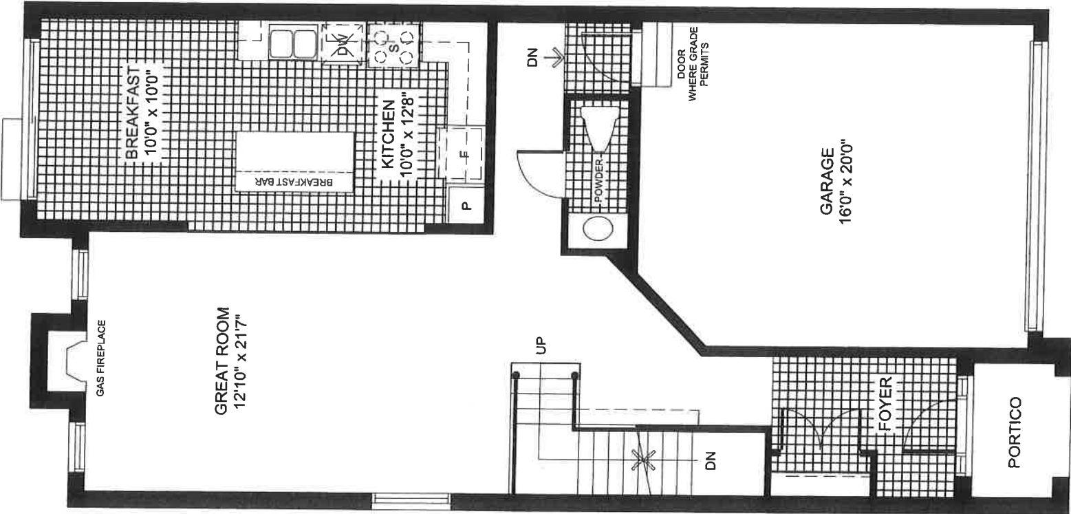
GROUND FLOOR ELEVATION 'B'
