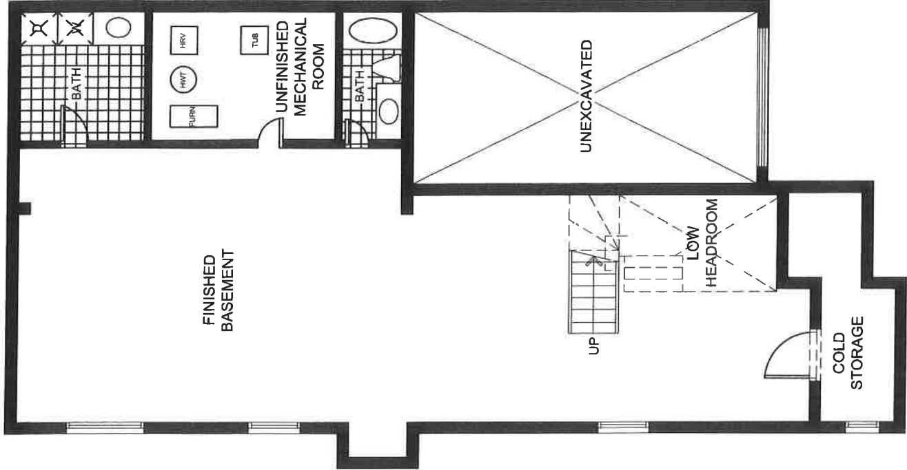
BASEMENT ELEVATION 'B'
