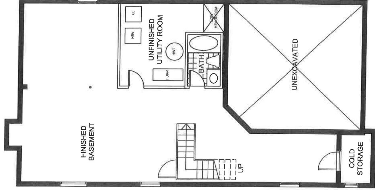
BASEMENT ELEVATION 'A'
