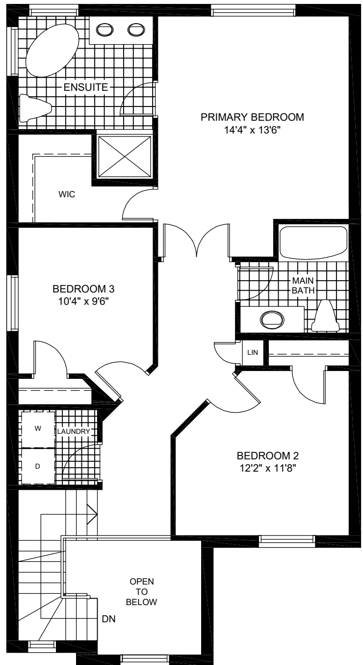
SECOND FLOOR ELEVATION 'B'
