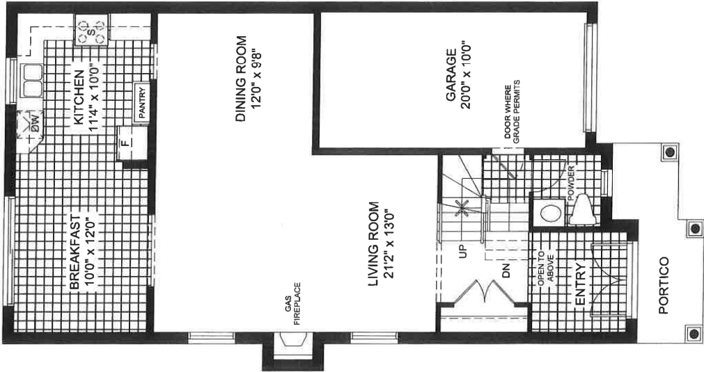
GROUND FLOOR ELEVATION 'B'
