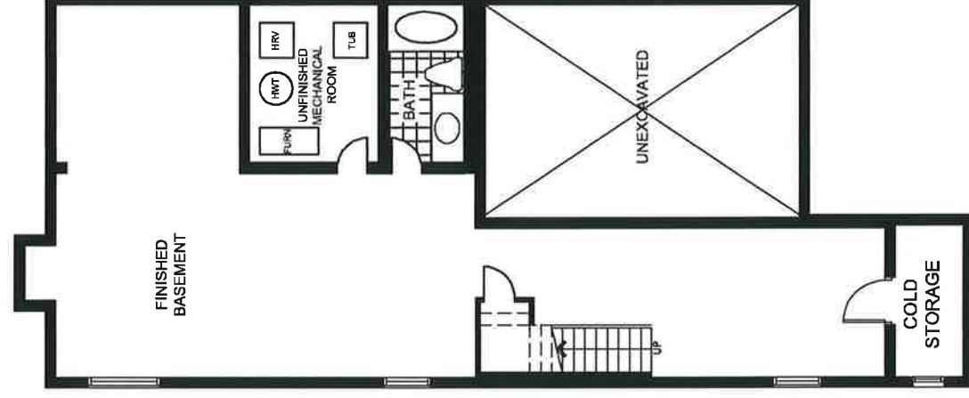
BASEMENT ELEVATION 'A'
