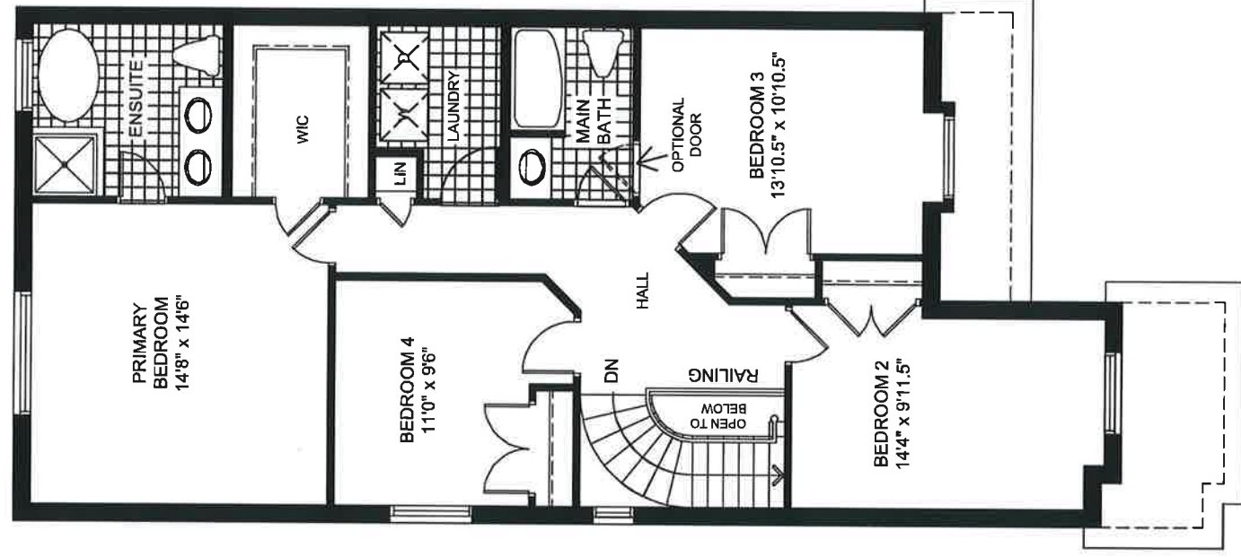
SECOND FLOOR ELEVATION 'B'
