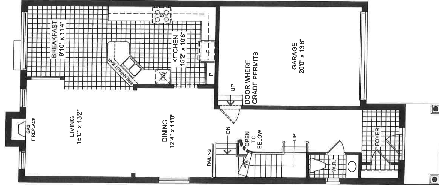
GROUND FLOOR ELEVATION 'A'
