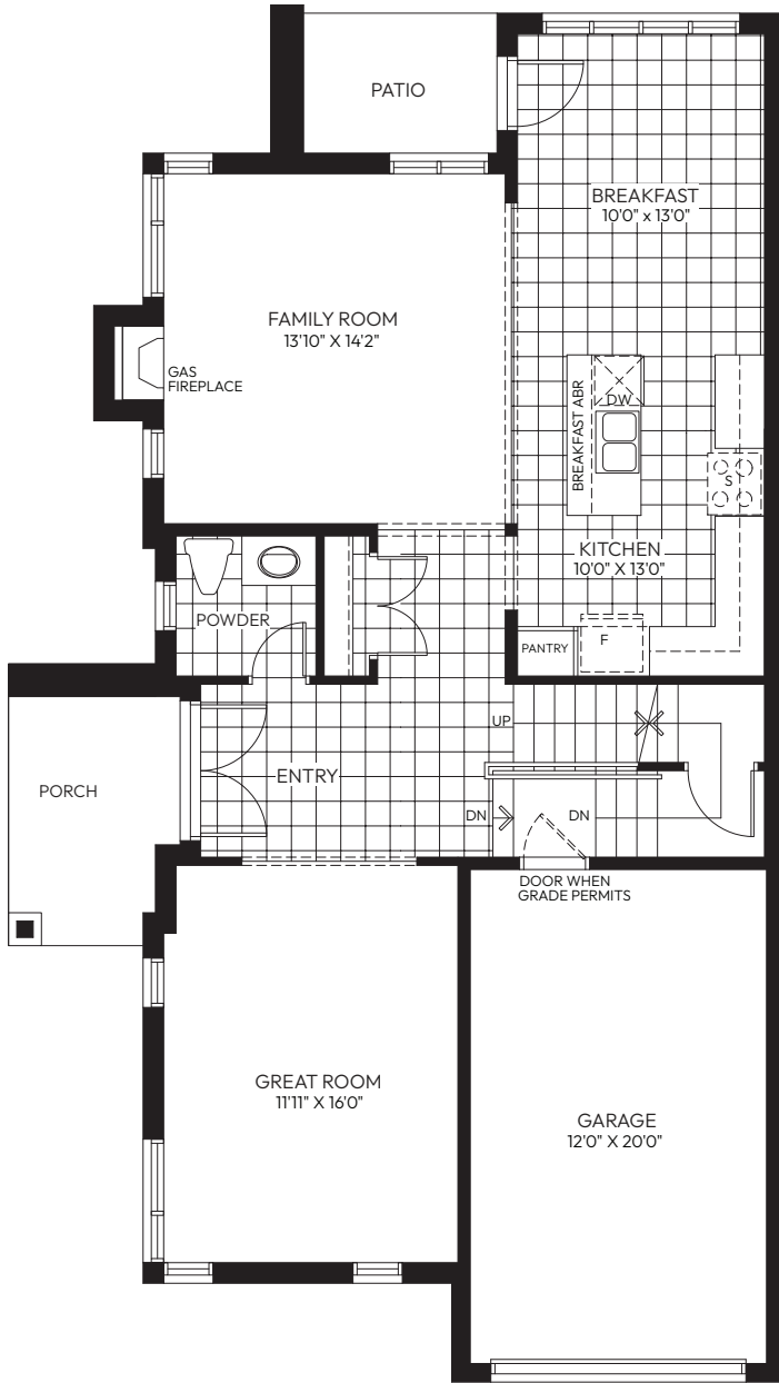
GROUND FLOOR - ELEVATION B
