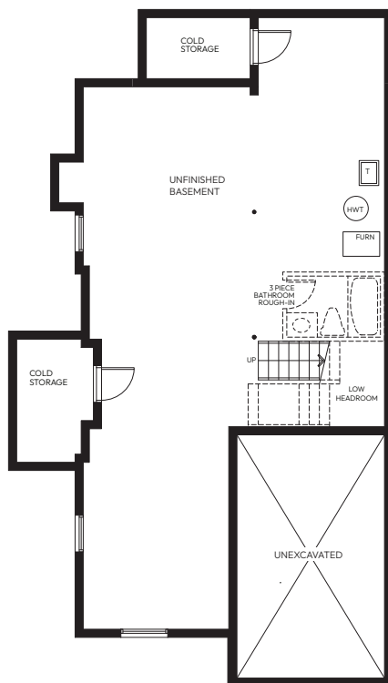
BASEMENT - ELEVATION B
